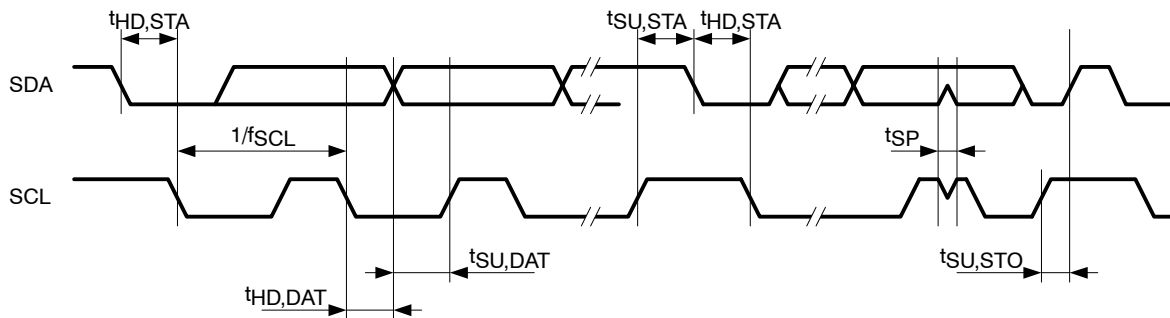
Figure 35. I2C Mode Timing
