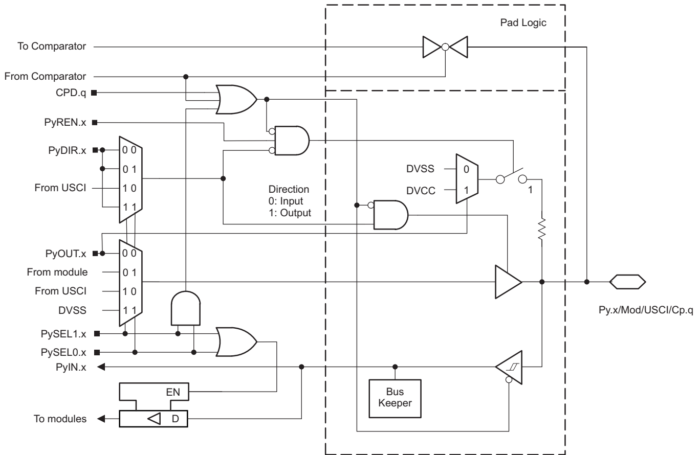
Figure 6-16. Py.x/Mod/USCI/Cp.q Pin Schematic
