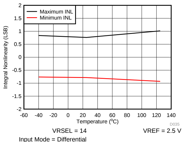
Figure 5-62. INL vs Temperature
