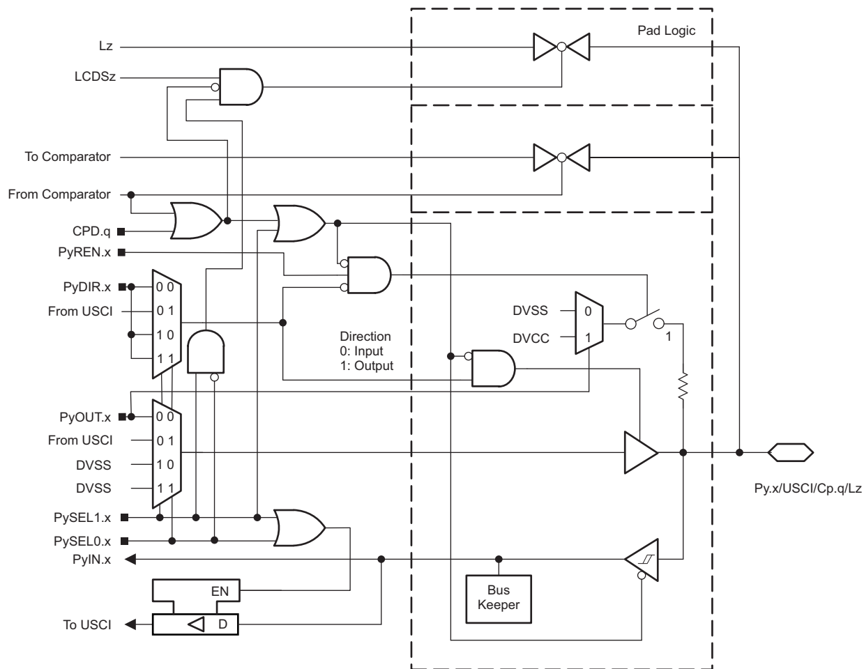
Figure 6-15. Py.x/USCI/Cp.q Pin Schematic
