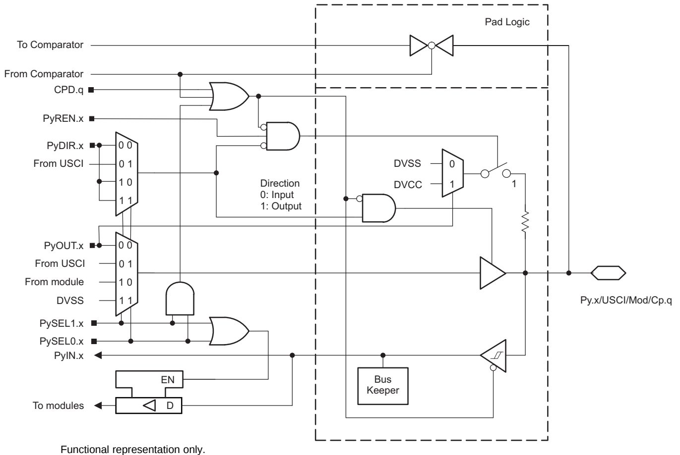
Figure 6-17. Py.x/USCI/Mod/Cp.q Pin Schematic
