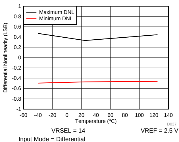
Figure 5-64. DNL vs Temperature
