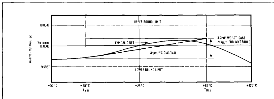
Figure 3. MX2700 Output Voltage Drift
