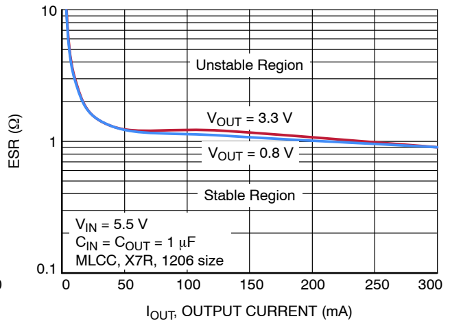
Figure 34. Output Capacitor ESR vs. Output Current
