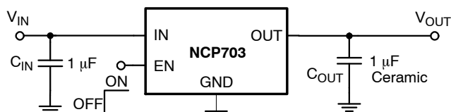
Figure 1. Typical Application Schematic
