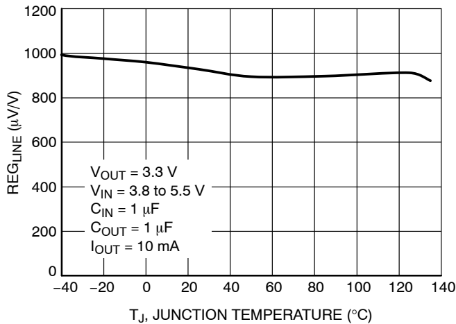
Figure 19. Line Regulation vs. Temperature – 3.3 V
