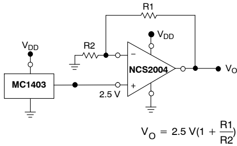
Figure 31. Voltage Reference
