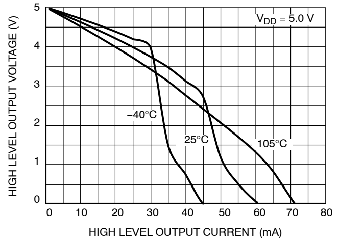
Figure 8. V_{OH} vs. I_{out}
