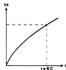
Slow-Start Voltage
