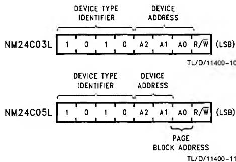
FIGURE 4. Slave Addresses
