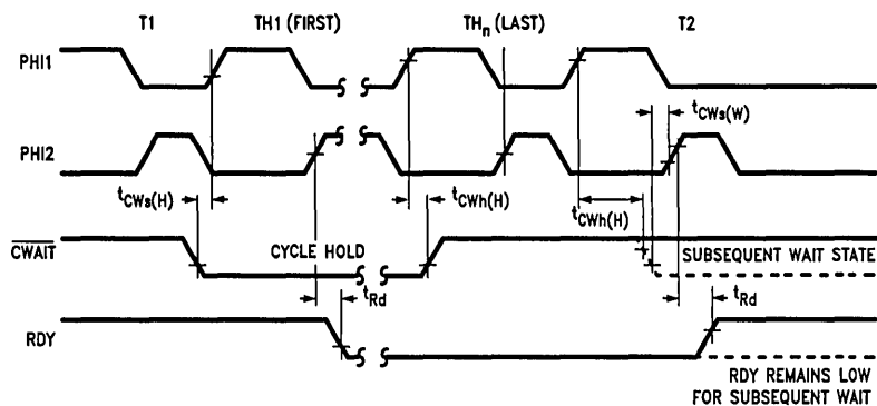
FIGURE 2-8. Cycle Hold
