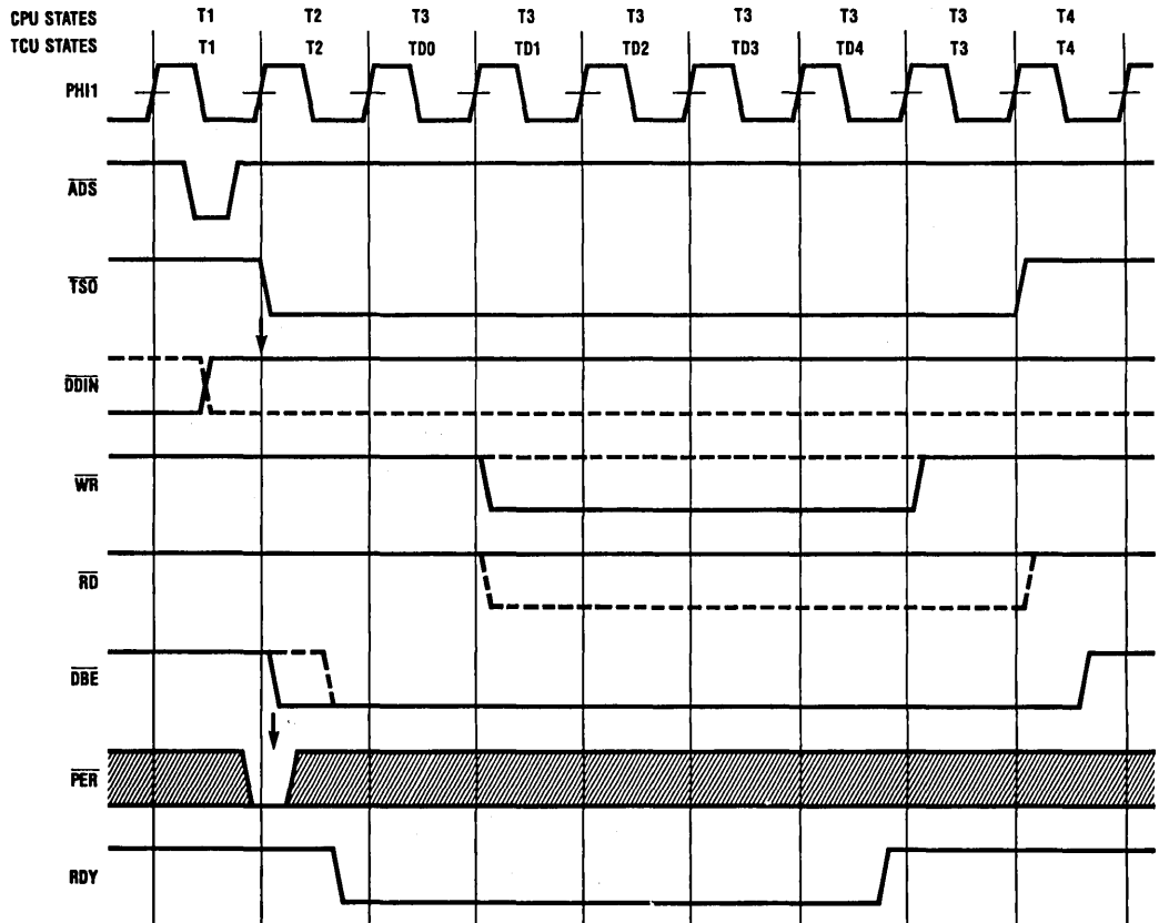
FIGURE 1-10. Peripheral Cycle
