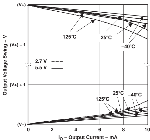
OFFSET VOLTAGE SWING vs OUTPUT CURRENT
