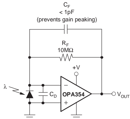
Figure 8. Transimpedance Amplifier
