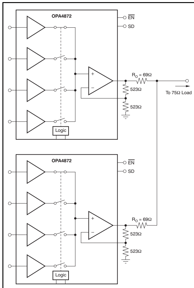
Figure 31. 8-to-1 Video Multiplexer
