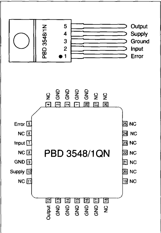
Figure 4. Pin descriptions.
