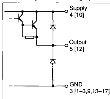
Figure 16. Output stage.
