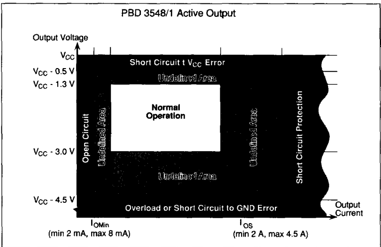
Figure 5. Error state vs. output voltage and output current, active output ( 0V \leq V_{IN} \leq 0.8V , 5V < V_{CC} < 40V and -40^{\circ}C < T_J < +100^{\circ}C )
