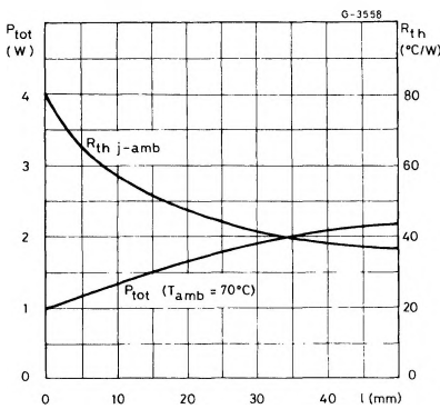
Figure 11 : Max. Dissippable Power and Junction to Ambient Thermal Resistance vs. size "α".
