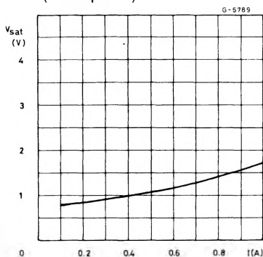
Figure 8 : Sink sat. Voltage vs. Output Current.
