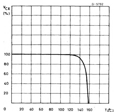
Figure 9 : Comparator threshold vs. Junction Temperature.
