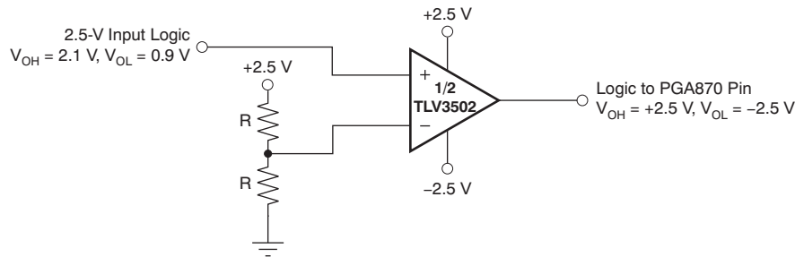
Figure 47. Comparator Circuit to Shift Logic Signals to PGA870 Operated on Split \pm 2.5 -V Supplies
