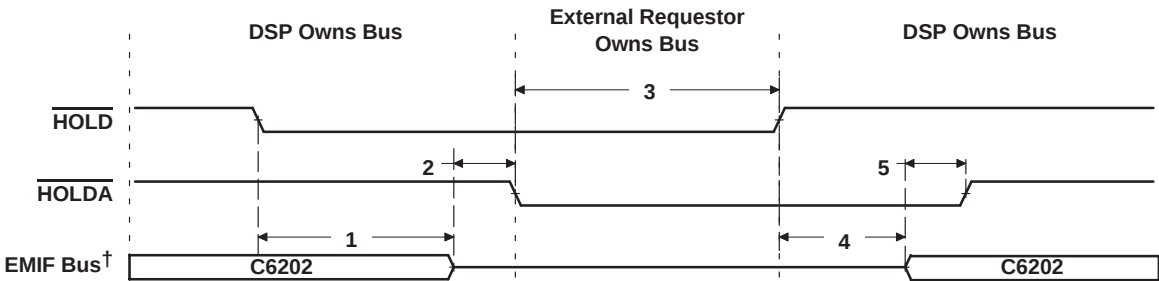
Figure 28. HOLD/HOLDA Timing
