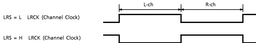
Figure 3a LRCK Polarity Setting Example in 2 ch Mode
