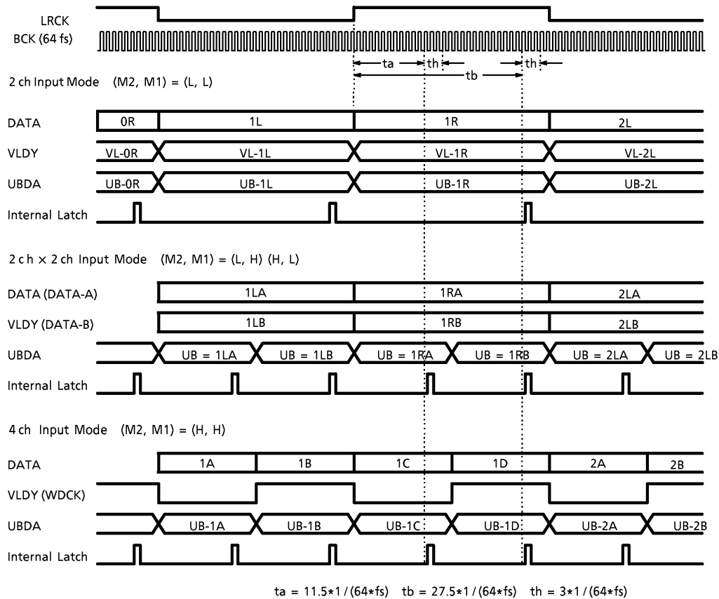
Figure 2 V and U Bit Input Timing Chart
