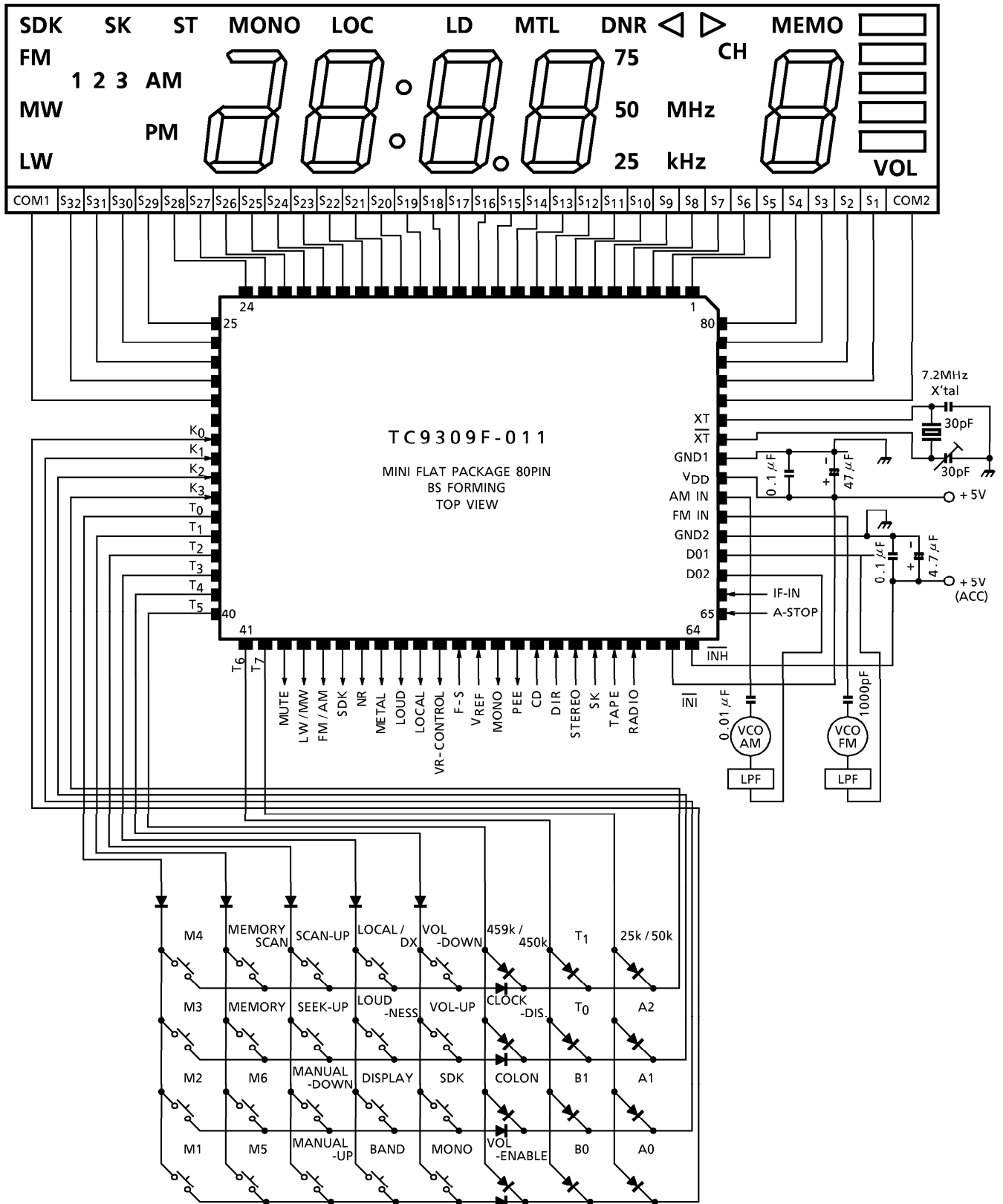
TC9309F-011 Layout
