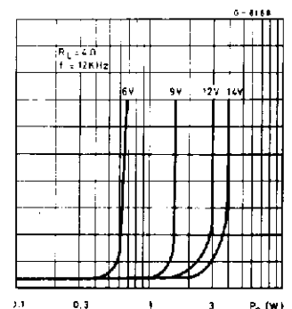
Figure 8. Distortion vs. output power
