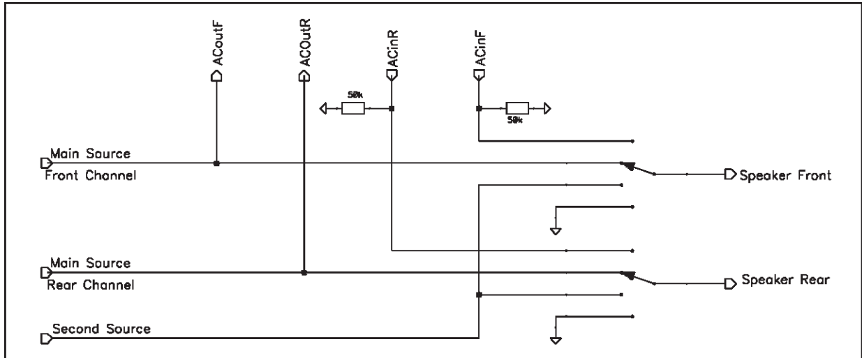
Figure 19. Output Selector
