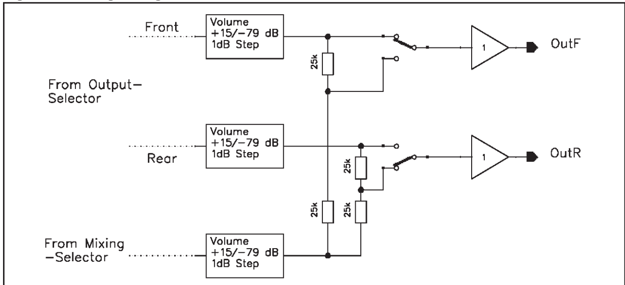
Figure 20. Mixing Configuration
