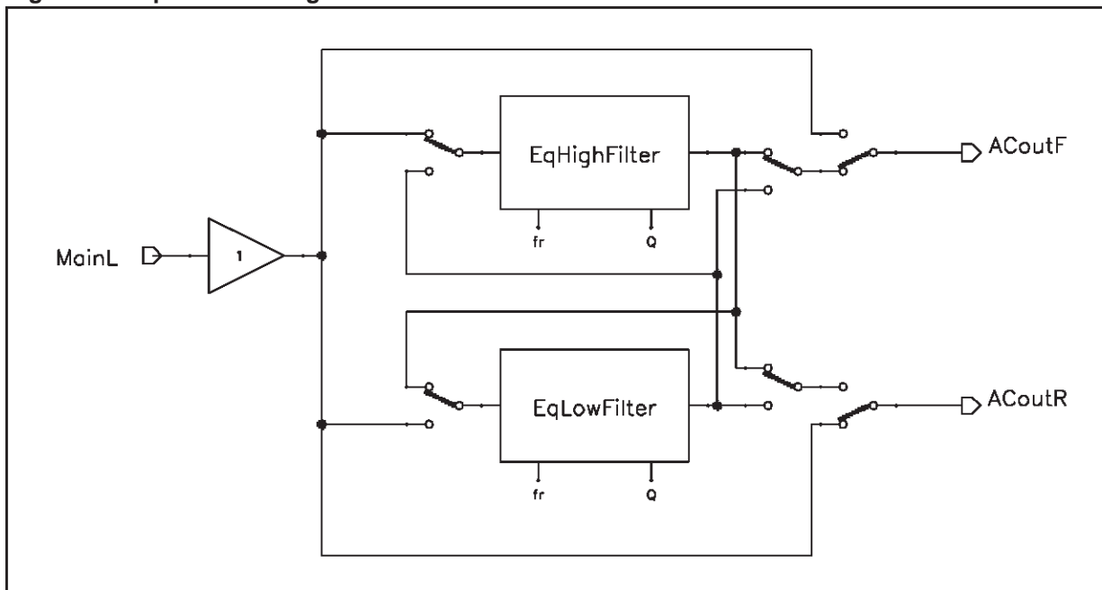
Figure 13. Equalizer Configuration
