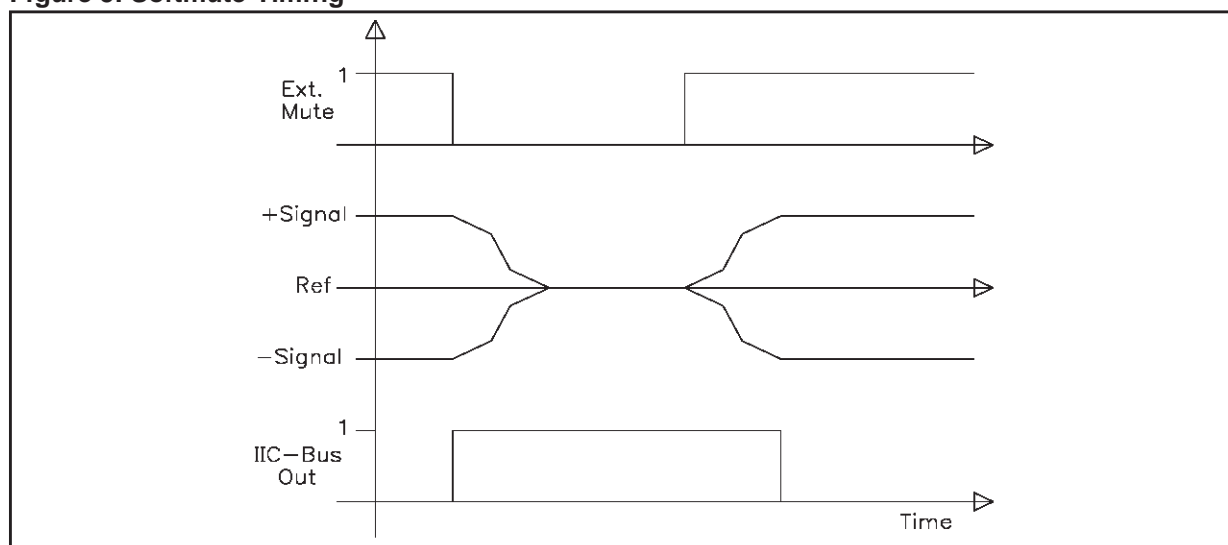
Figure 5. Softmute-Timing
