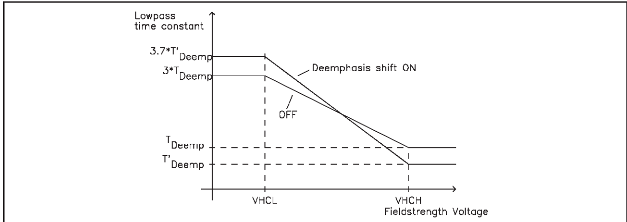
Figure 30. Highcut characteristics
