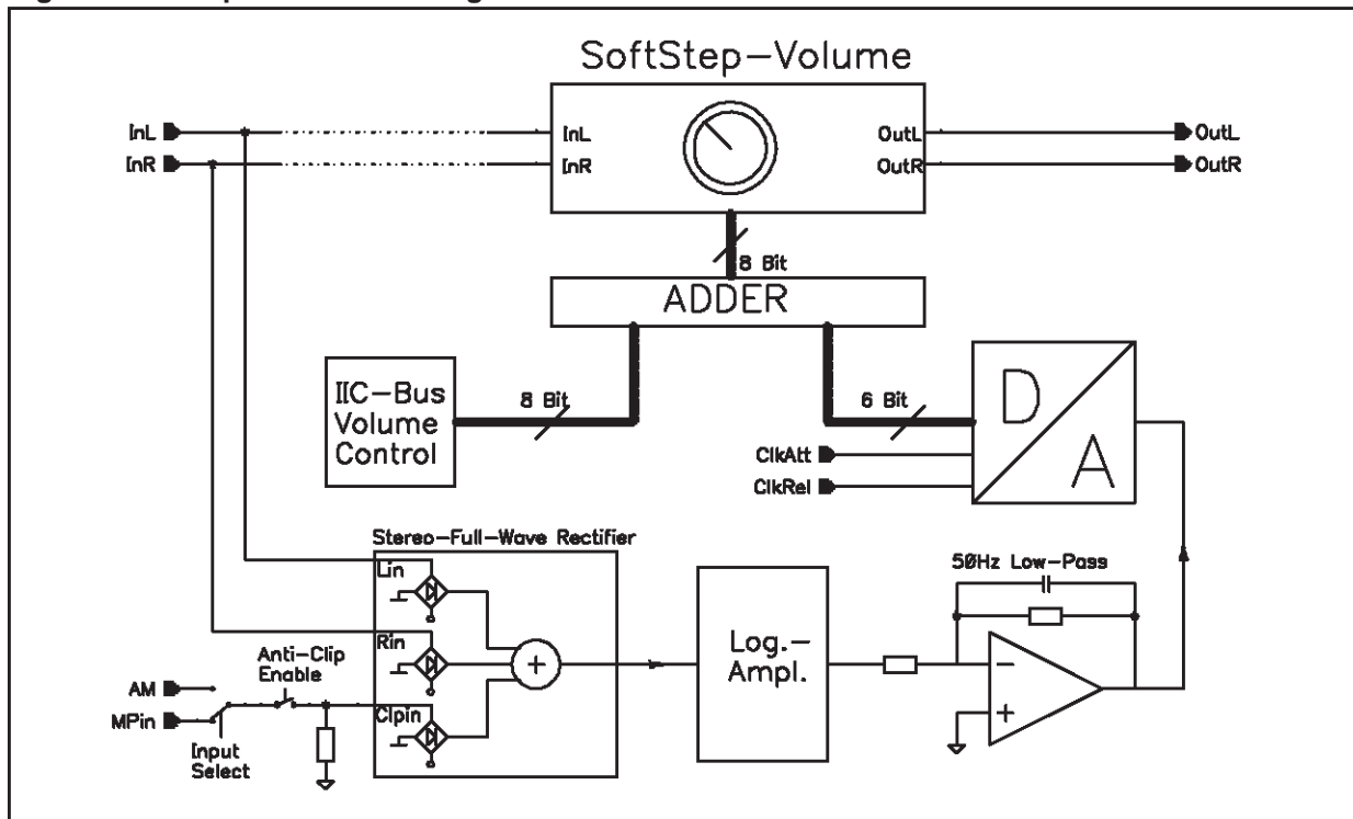
Figure 17. Comander Block Diagram
