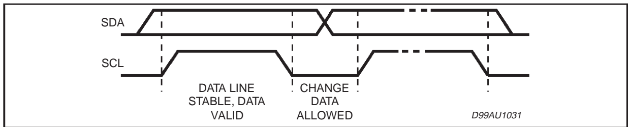
Figure 23: Timing Diagram on the I 2 C BUS
