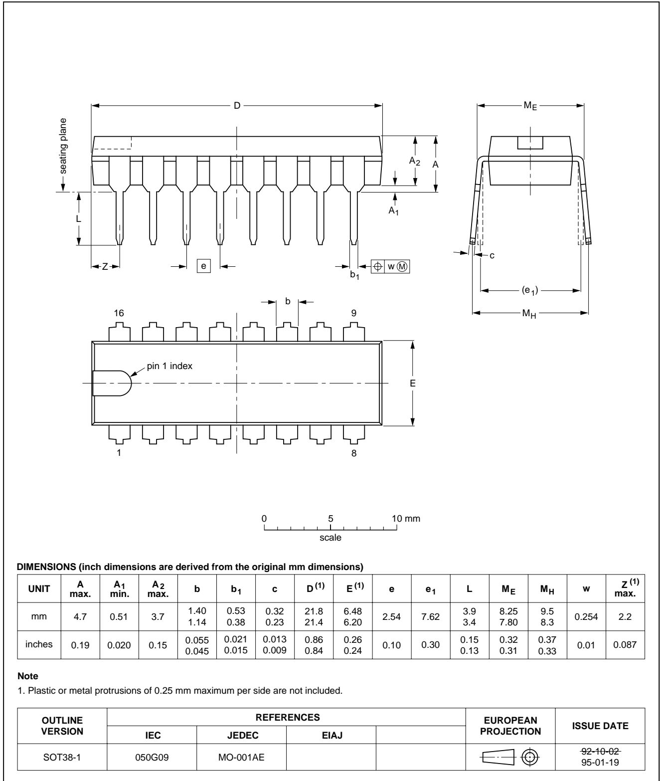
Fig 4. DIP16 package outline.
