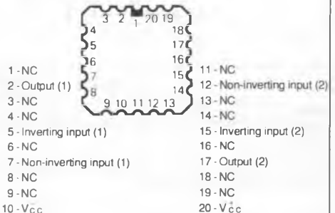
LCC20
