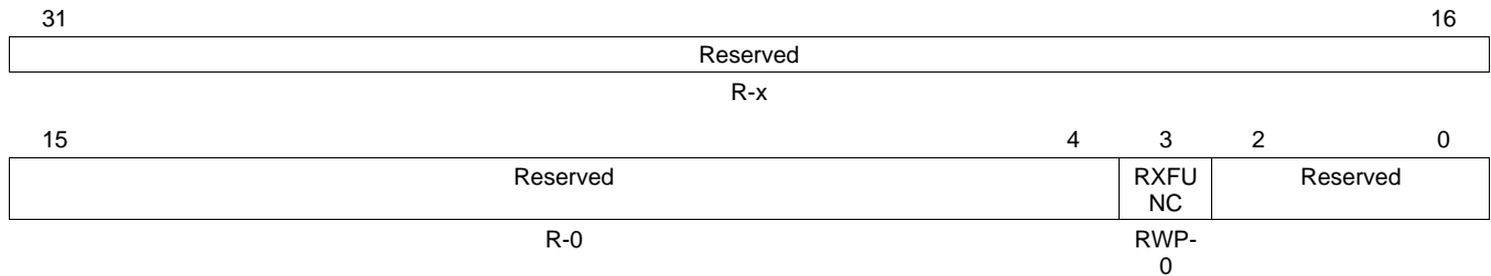
Figure 27. RX I/O Control Register (CANRIOIC)
