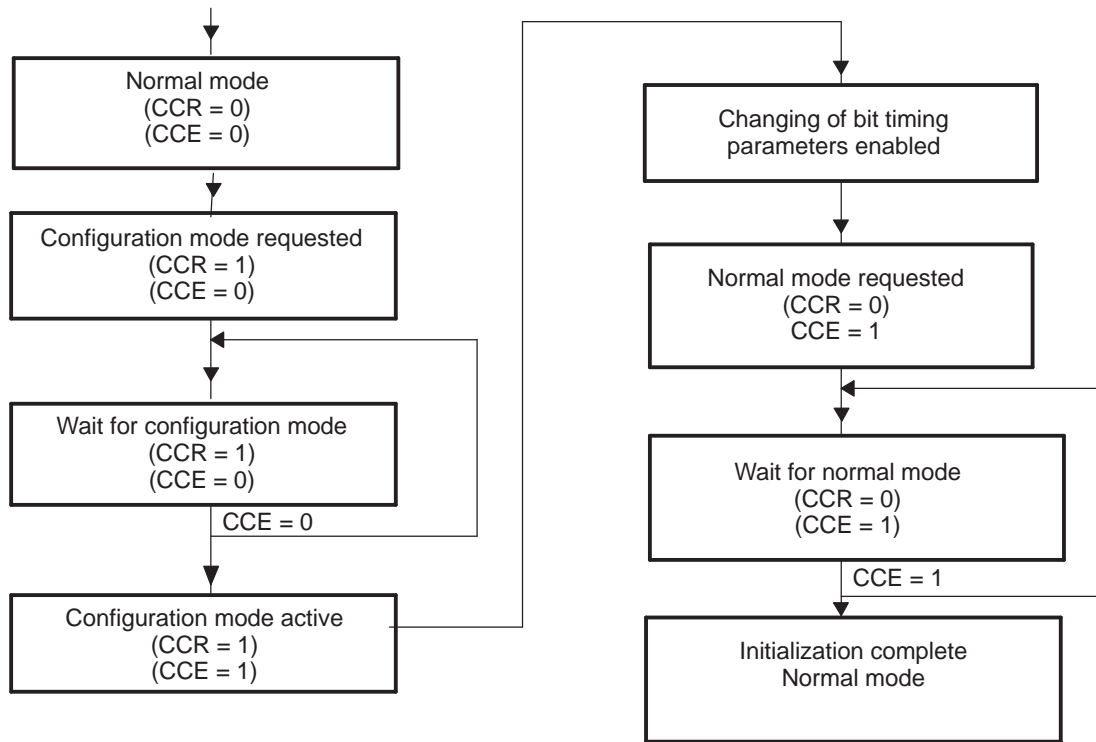
Figure 40. Initialization Sequence
