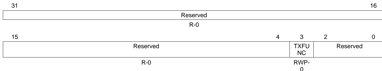
Figure 26. TX I/O Control Register (CANTIOC)
