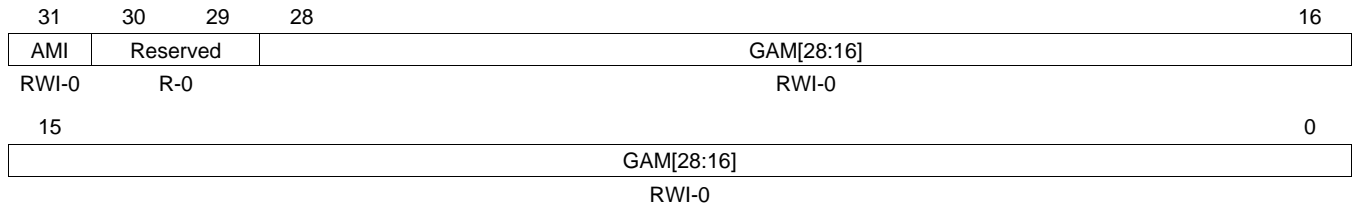
Figure 14. Global Acceptance Mask Register (CANGAM)
