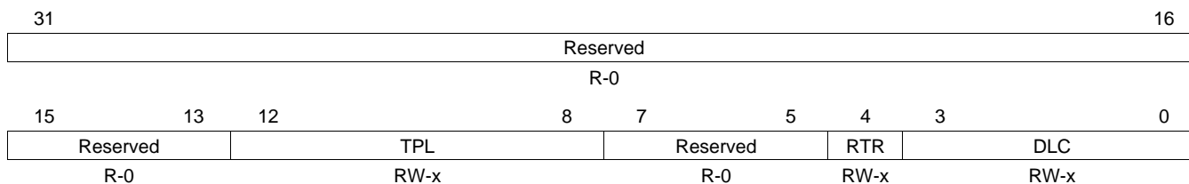
Figure 34. Message-Control Register (MSGCTRL)
