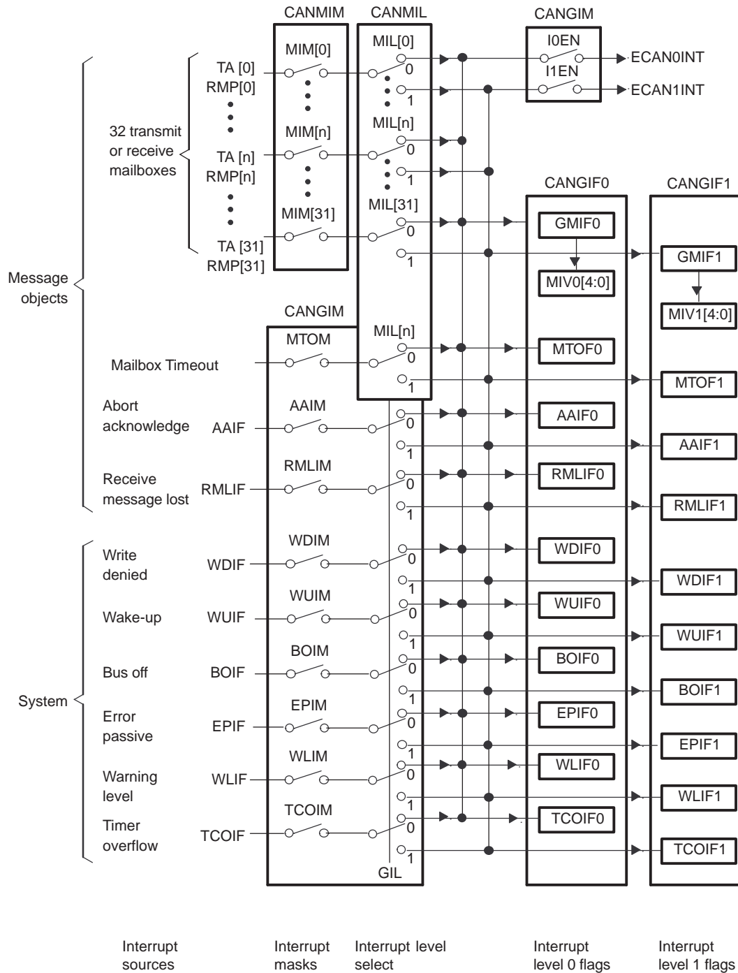
Figure 42. Interrupts Scheme
