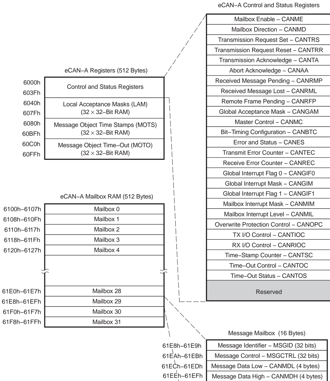
Figure 4. eCAN-A Memory Map
