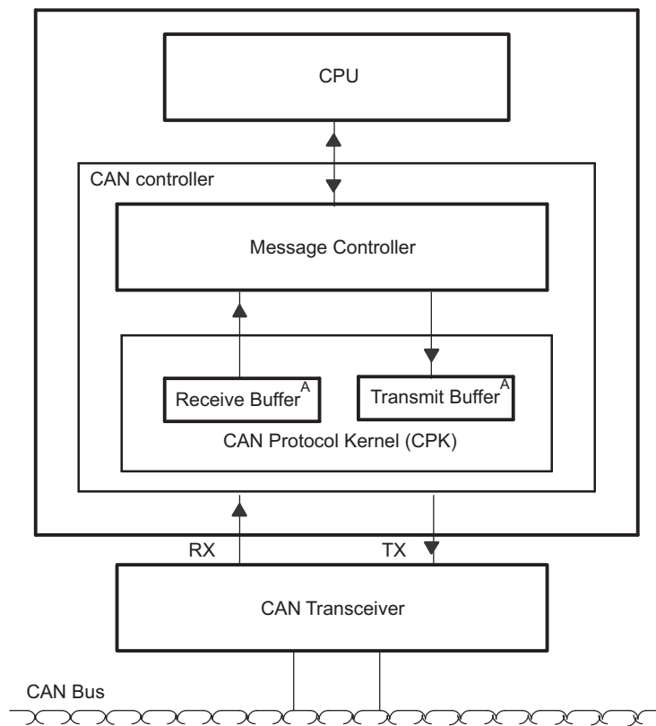
Figure 3. Architecture of the eCAN Module
