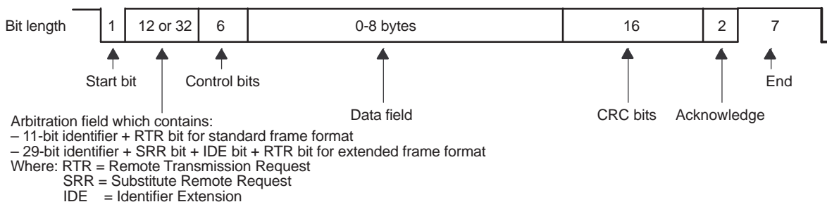
Figure 2. CAN Data Frame
