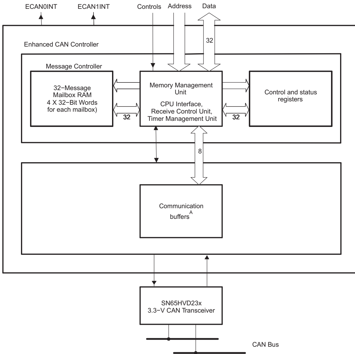
Figure 1. eCAN Block Diagram and Interface Circuit
