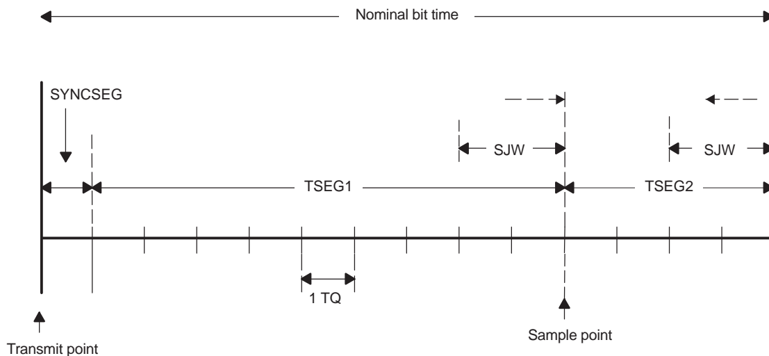
Figure 41. CAN Bit Timing
