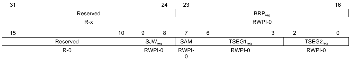
Figure 16. Bit-Timing Configuration Register (CANBTC)
