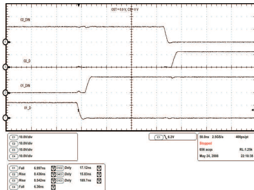
Figure 29. Output Waveforms During First Half Switching Cycle at V_{CS} = 0\text{ V} and V_{OST} = 1\text{ V}
