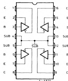
ULN2075B ULN2077B
