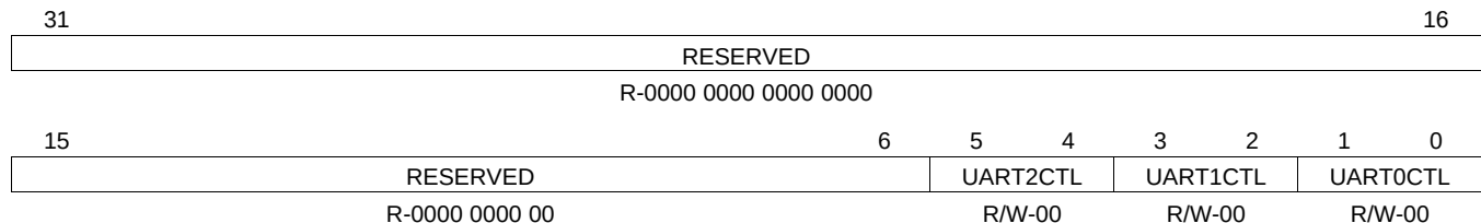
Figure 3-19. PINMUX1 Register
