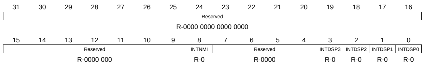
Figure 3-20. DSPINT Status Register [0x01C4 0060]
