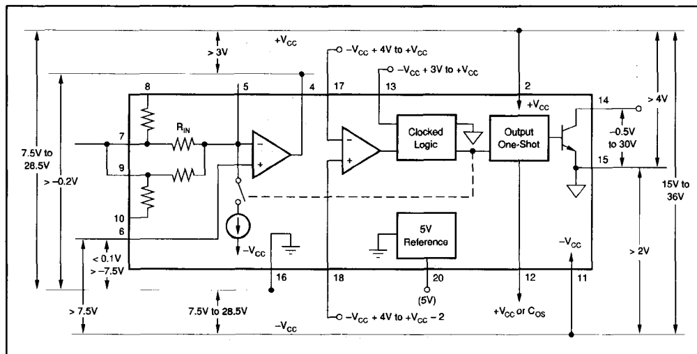
FIGURE 6. Relationships of Allowable Voltages.
