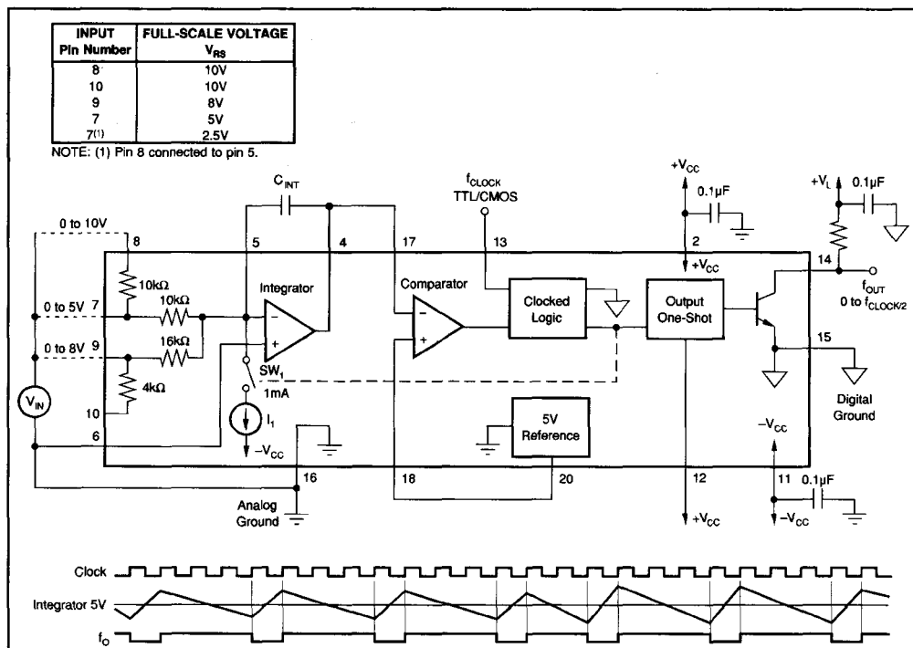
FIGURE 1. Basic Voltage-to-Frequency Operations.
