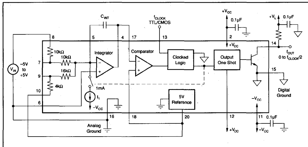
FIGURE 2. Offset for Bipolar Input Voltages.
