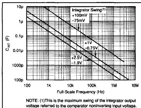
FIGURE 3. Integrator Capacitor Selection Graph.
