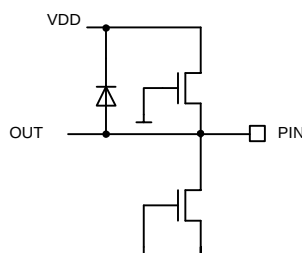
Fig. 4-17: Analog Output Pins: CVBSO1...CVBSO3
