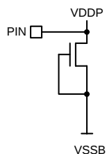
Fig. 4-7: Supply Pins (Power 3.3 V): VDDDACY , VDDDACU , VDDDACV , VDD33C , VDD33RGB , VDDP1 , VDDP2 , VDDP3
