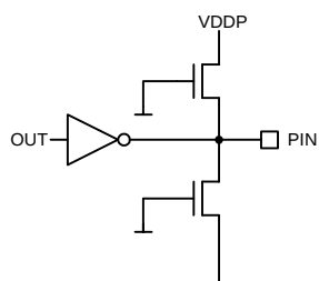
Fig. 4-10: Digital Output Pins: H50, V50, CLKOUT, HOUT, VOUT
