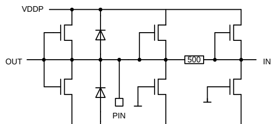
Fig. 4-13: Digital Input/Output Pins: 656IOX, 656CLK, 656HIN/CLKF20, 656VIN/BLANK
