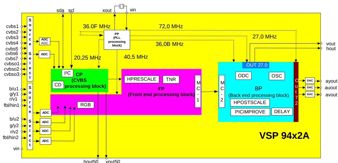
Fig. 3-1: I²C bus clock domains
