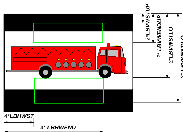
Fig. 2-28: Measurement Windows
