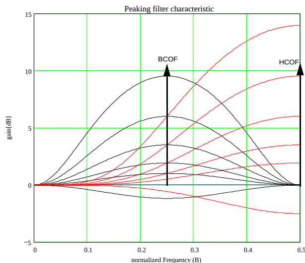
Fig. 2–33: Peaking filter: Bandpass and Highpass filter
