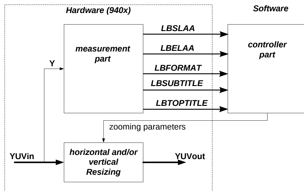
Fig. 2-27: HW/SW Partitioning
