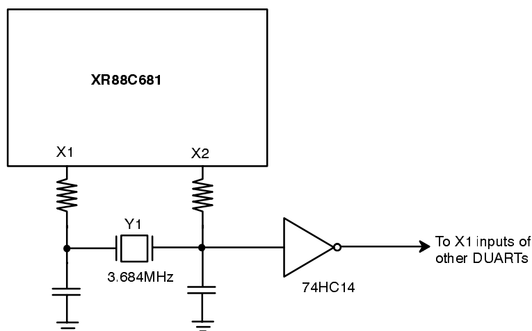
Figure 26. A Recommended Schematic to Drive Multiple DUARTs From the Same Crystal Oscillator.
