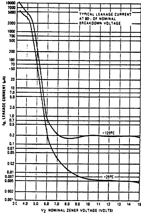
Figure 3 TYPICAL LEAKAGE CURRENT
