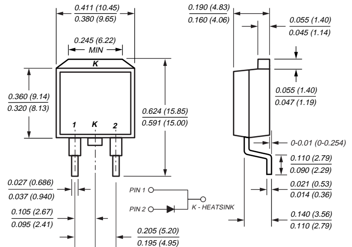
TO-263AB (MBRB7xx)
