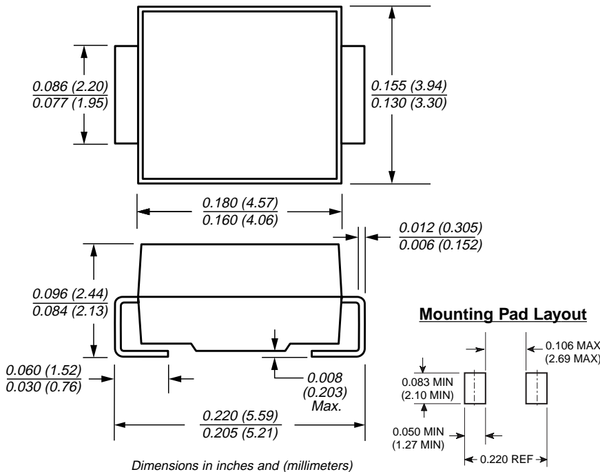
DO-214AA (SMB)
