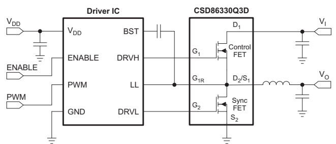
TYPICAL CIRCUIT
