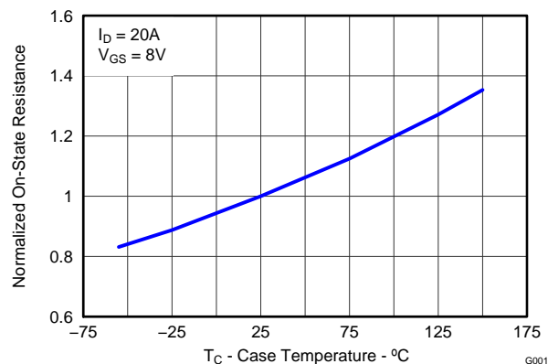
Figure 23. Sync MOSFET Normalized R_{DS(on)}
