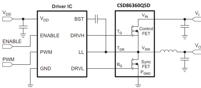
TYPICAL CIRCUIT
