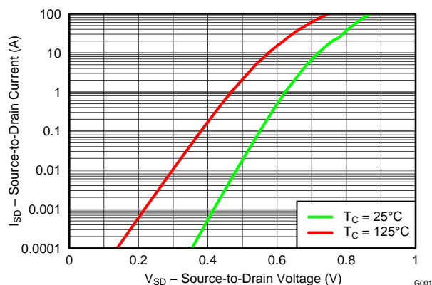
Figure 25. Sync MOSFET Body Diode
