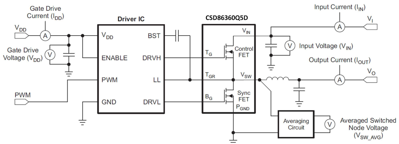
Figure 32. Typical Application
