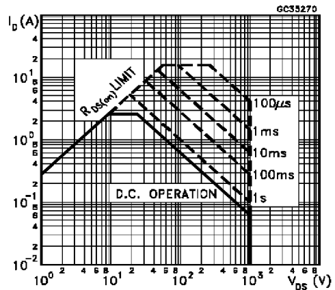
Safe Operating Areas For ISOWATT218
