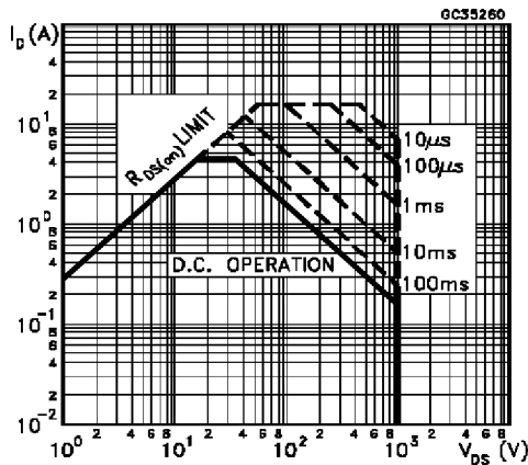
Safe Operating Areas For TO-218
