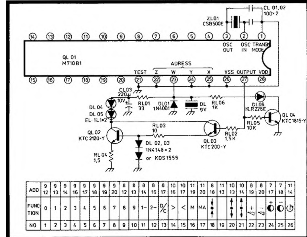
TRANSMITTER BOARD PW1620
