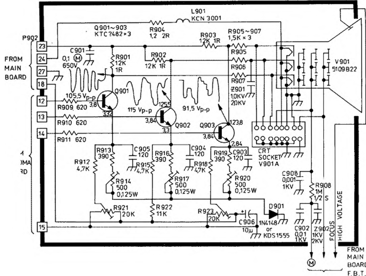
CRT SOCKET BOARD PW 1617
