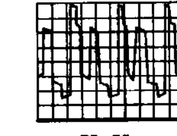
TP 35 ① 1 V/div DC 20 uS/div
