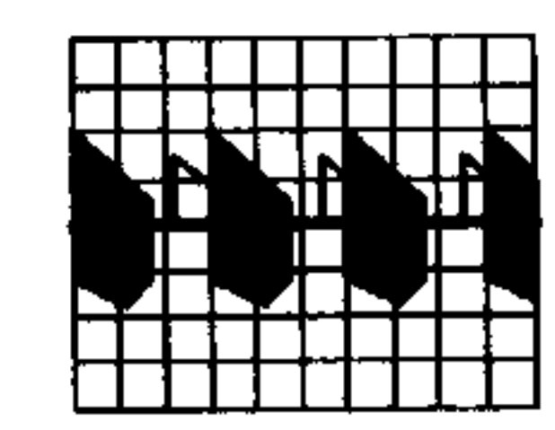
TP 28 ① 50 mV/div AC 20 uS/DIV
